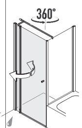
Swinging door attached on fixed part next to shortened side screen 11 door part, 1 fixed part
